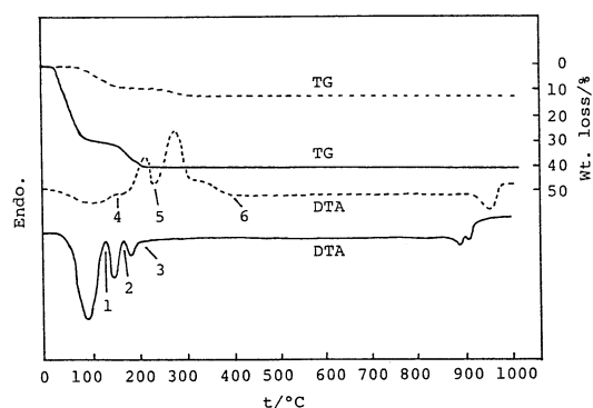
Fig. 1. TG and DTA curves of the imidodiphosphates. —: Na 4 P 2 O 6 NH·10H 2 O, ----: amorphous imidodiphosphate.
